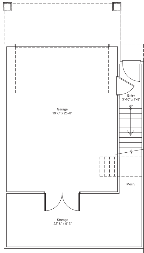
ENTRY FLOOR
